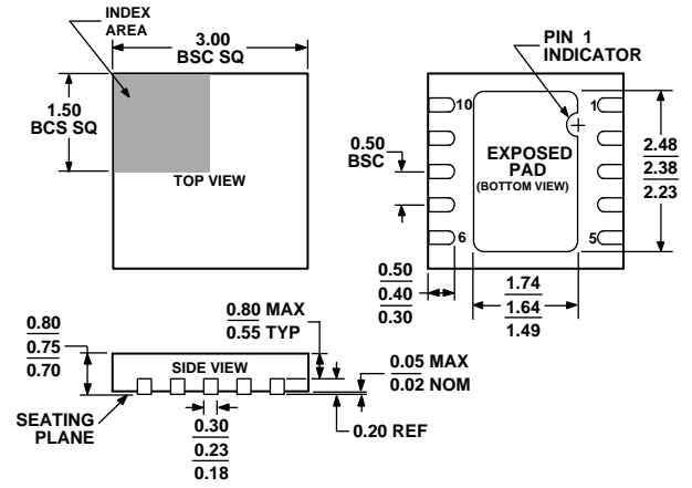
Figure 49. 10-Lead Lead Frame Chip Scale Package [LFCSP_WD]
